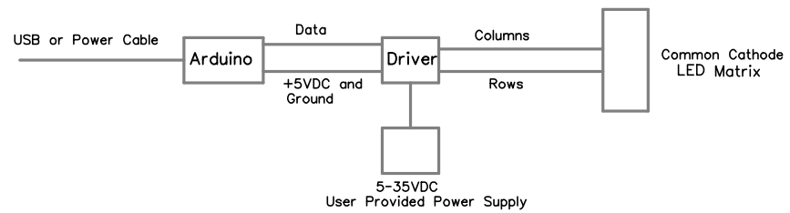
Block Diagram of HV LED Driver Shield
